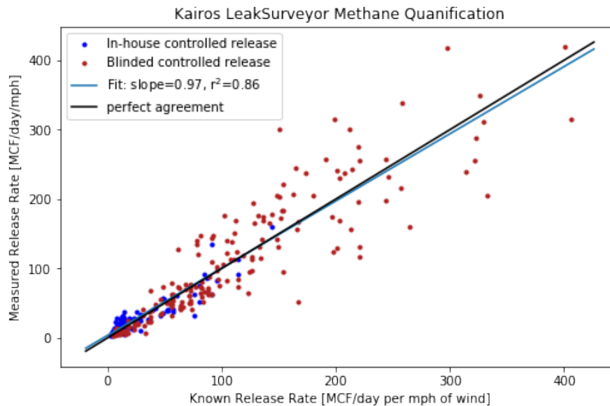
Figure 6: Quantification of methane release rate shown for controlled release data from nine different occasions in three different locations and on three different instruments. The best fit line shows excellent agreement with the line of perfect agreement.
