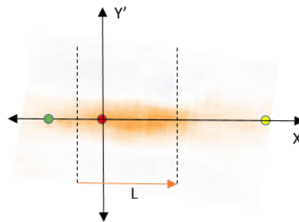
Figure 3: Excess Column Density map for the plume
